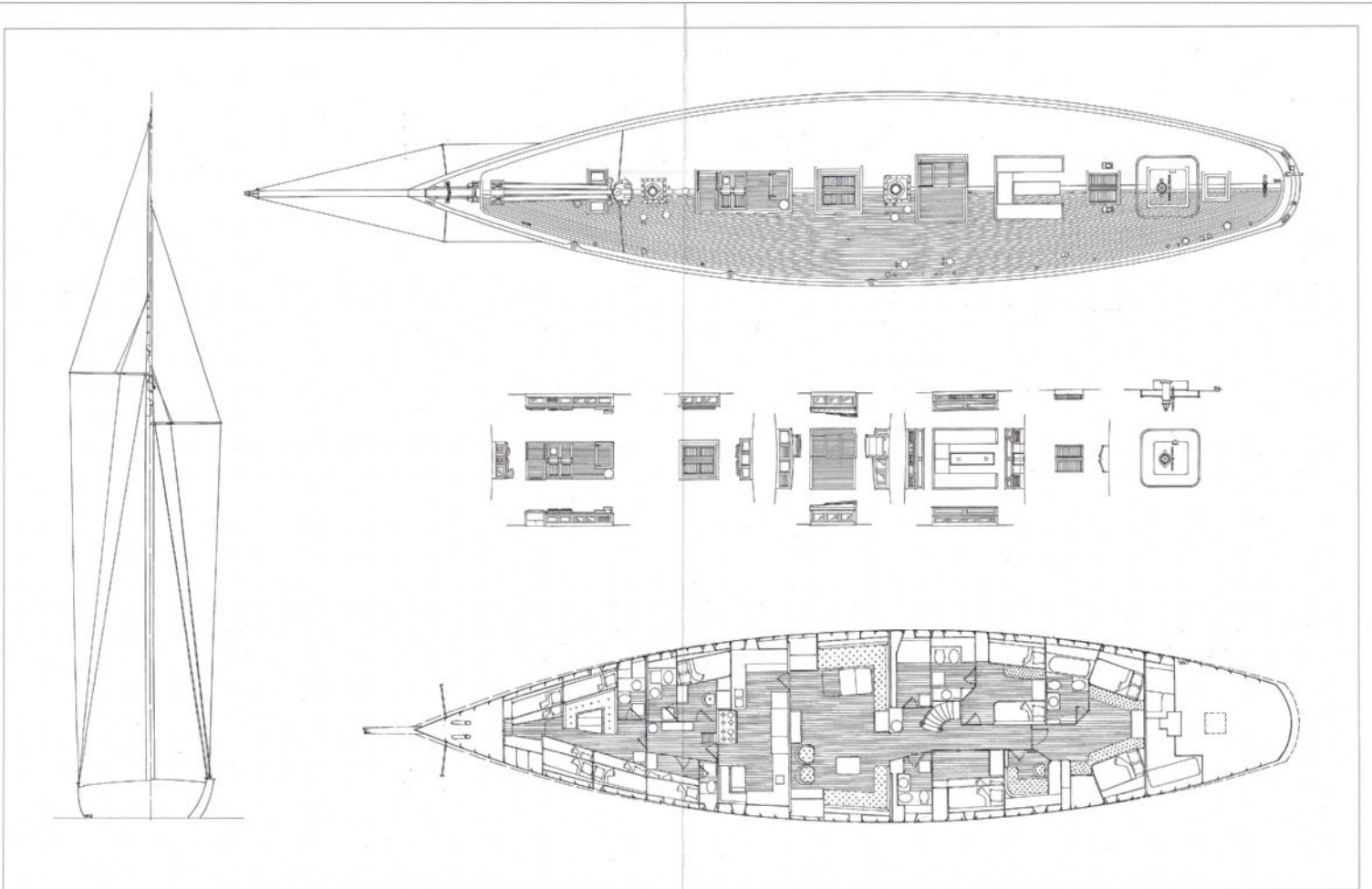
Detailed drawing of the accommodations, deck, and rigging of Mariette - 1995 version, by François Chevalier (©2010 François Chevalier)
